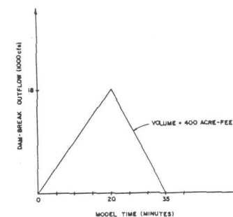
Figure 3. Study Dam-Break Outflow Hydrograph
