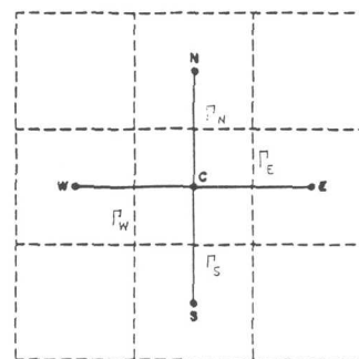
Figure 1. Grid Element Nodal Molecule
