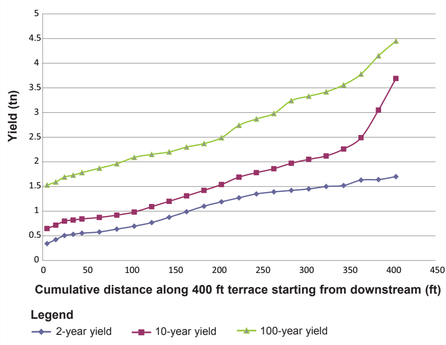
Figure 2 FLUVIAL-12 sediment yield along 400-foot terrace.
