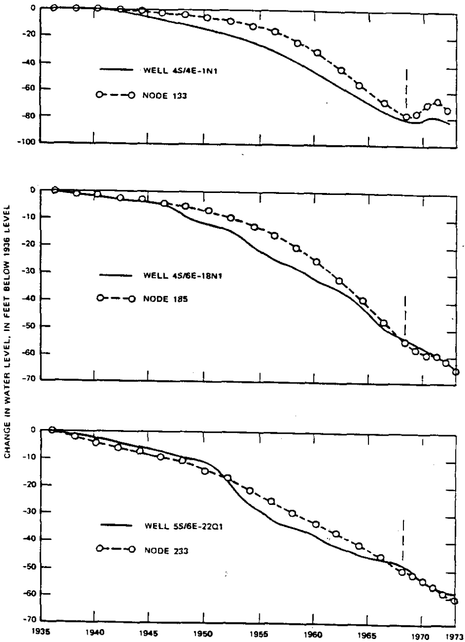
Figure 3.6: Comparison of measured and simulated water levels for Upper Coachella Valley groundwater basin model[14].
