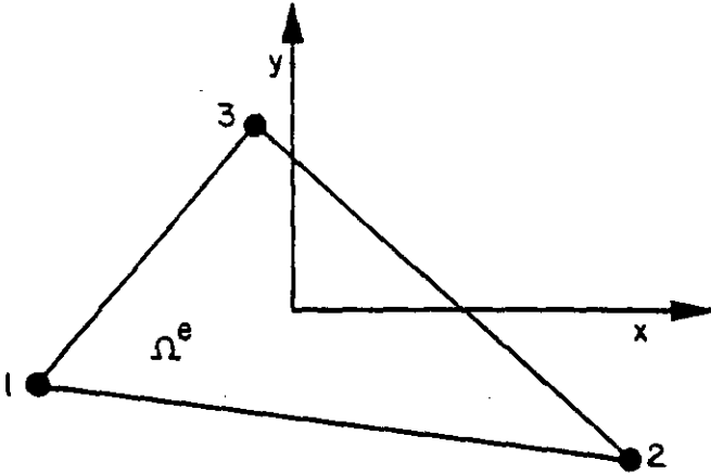
Figure 3.4: Finite-element triangle.
